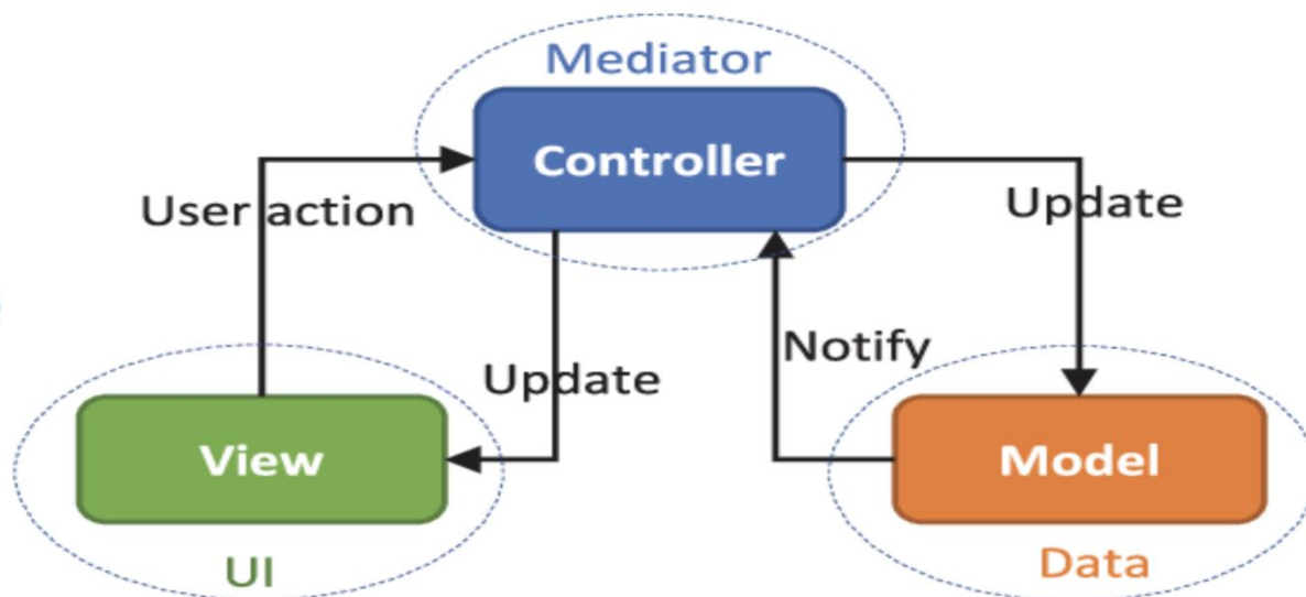
Model-View-Controller(MVC) design pattern.
